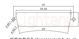
板前安装开孔 (Front Install Cutout)
